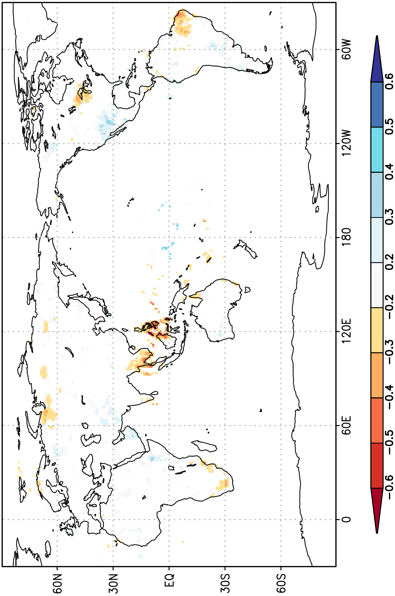
corr Apr rel NINO3.4 index with Apr GPCC+ precipitation 1901:2022 p<10%
