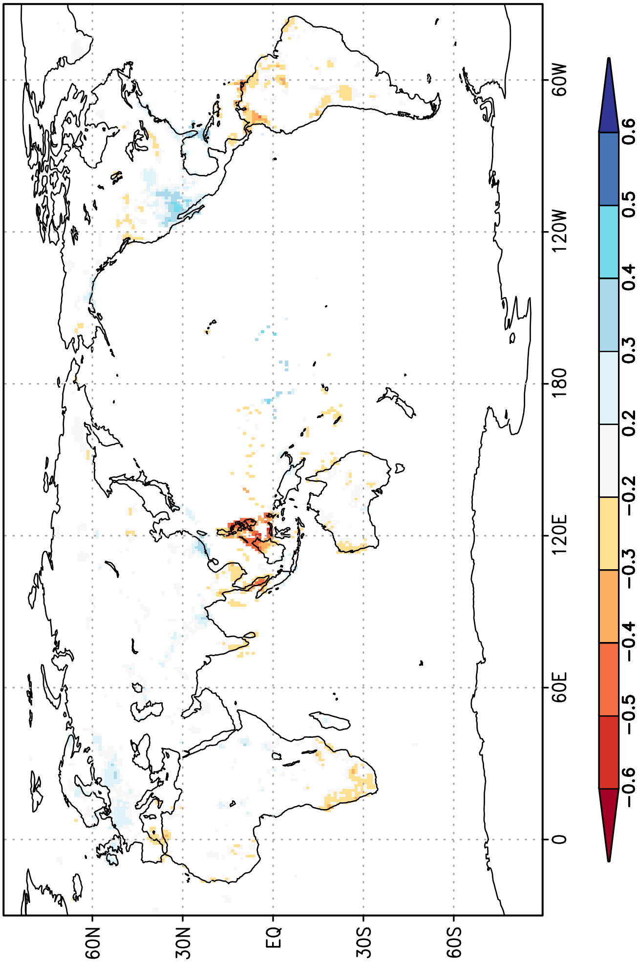
corr Mar rel NINO3.4 index with Mar GPCC+ precipitation 1901:2022 p < 10\%
