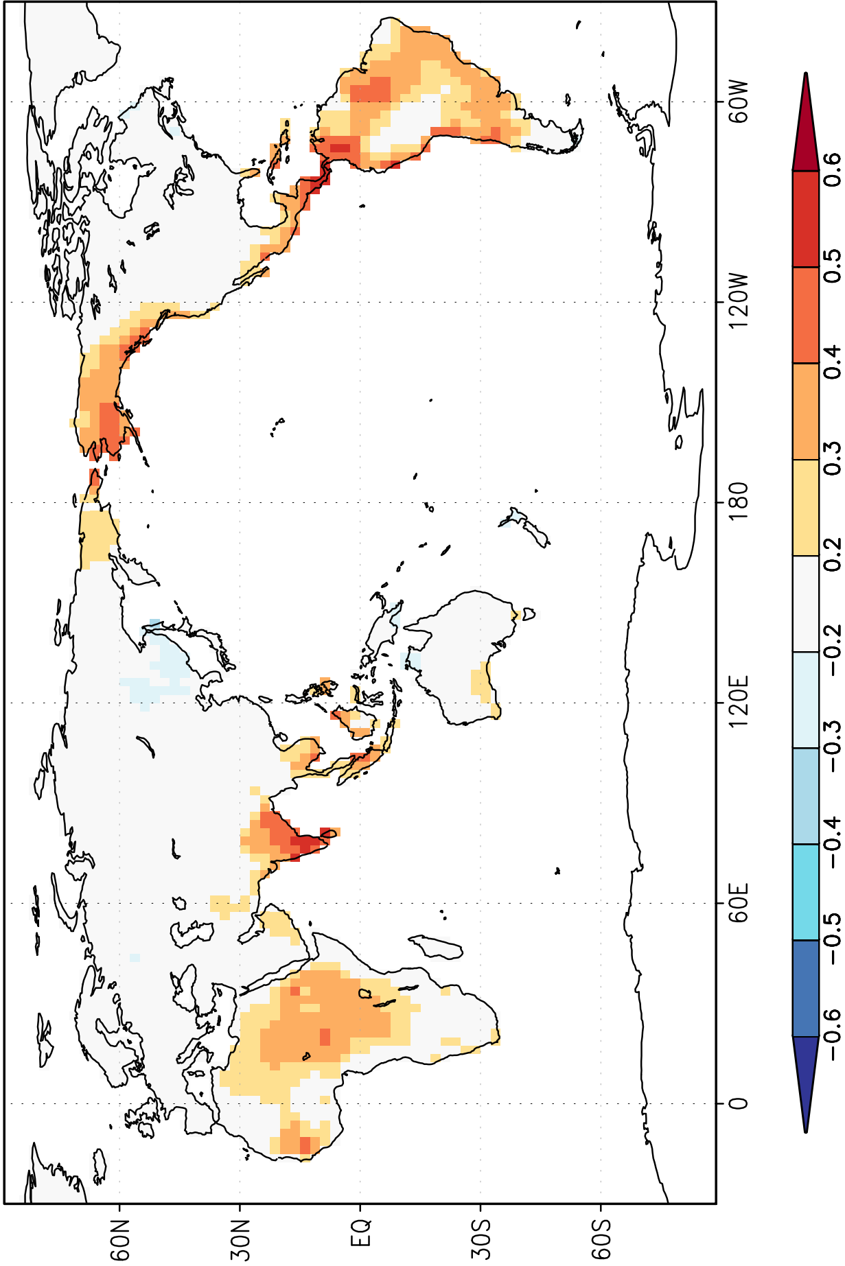
corr Jun-Aug NINO3.4 index with Jun-Aug CRU TS3.22 temperature 1901:2013
