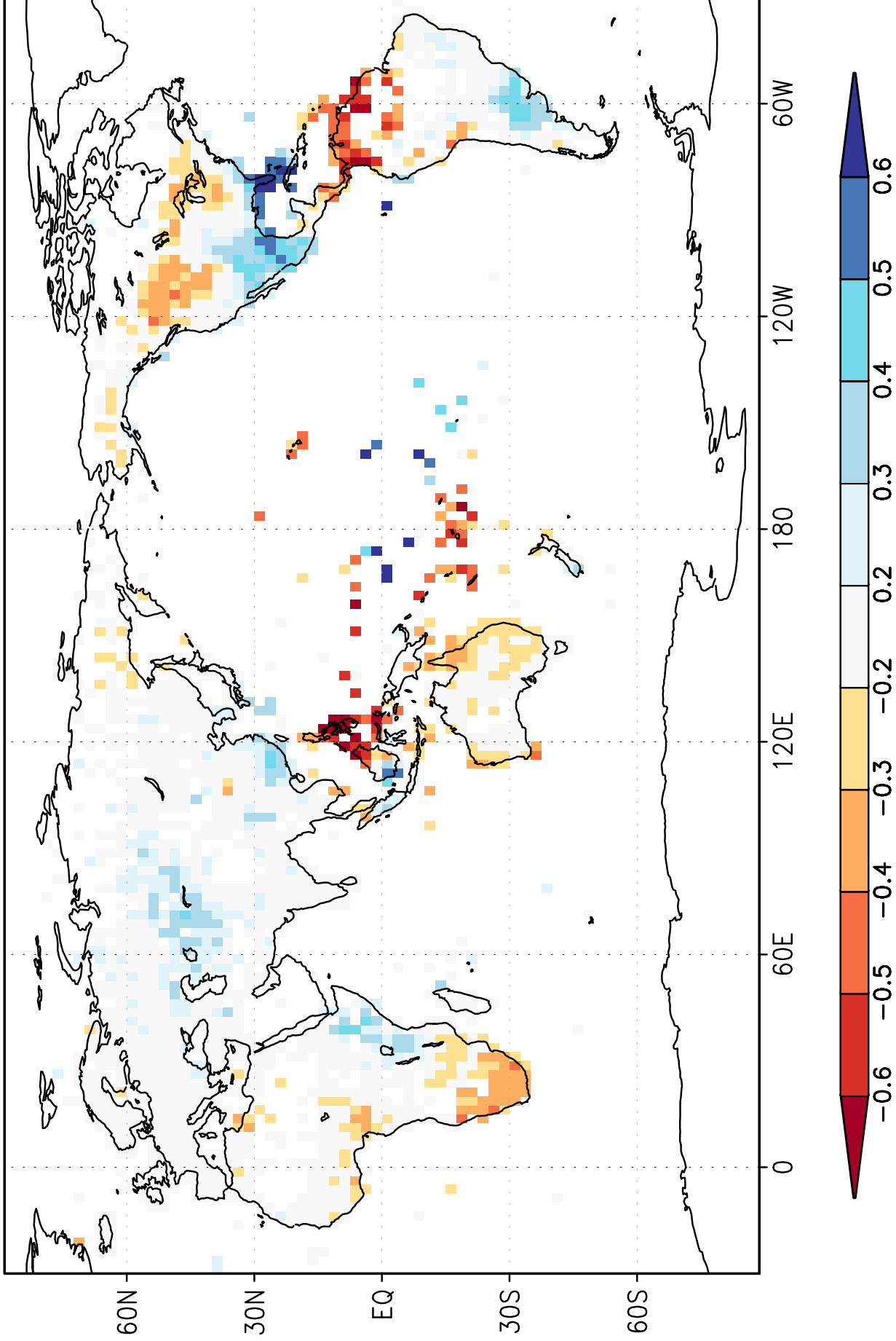
corr Dec-Feb NINO3.4 index with Dec-Feb GPCC V7 2.5 precipitation 1901:2013
