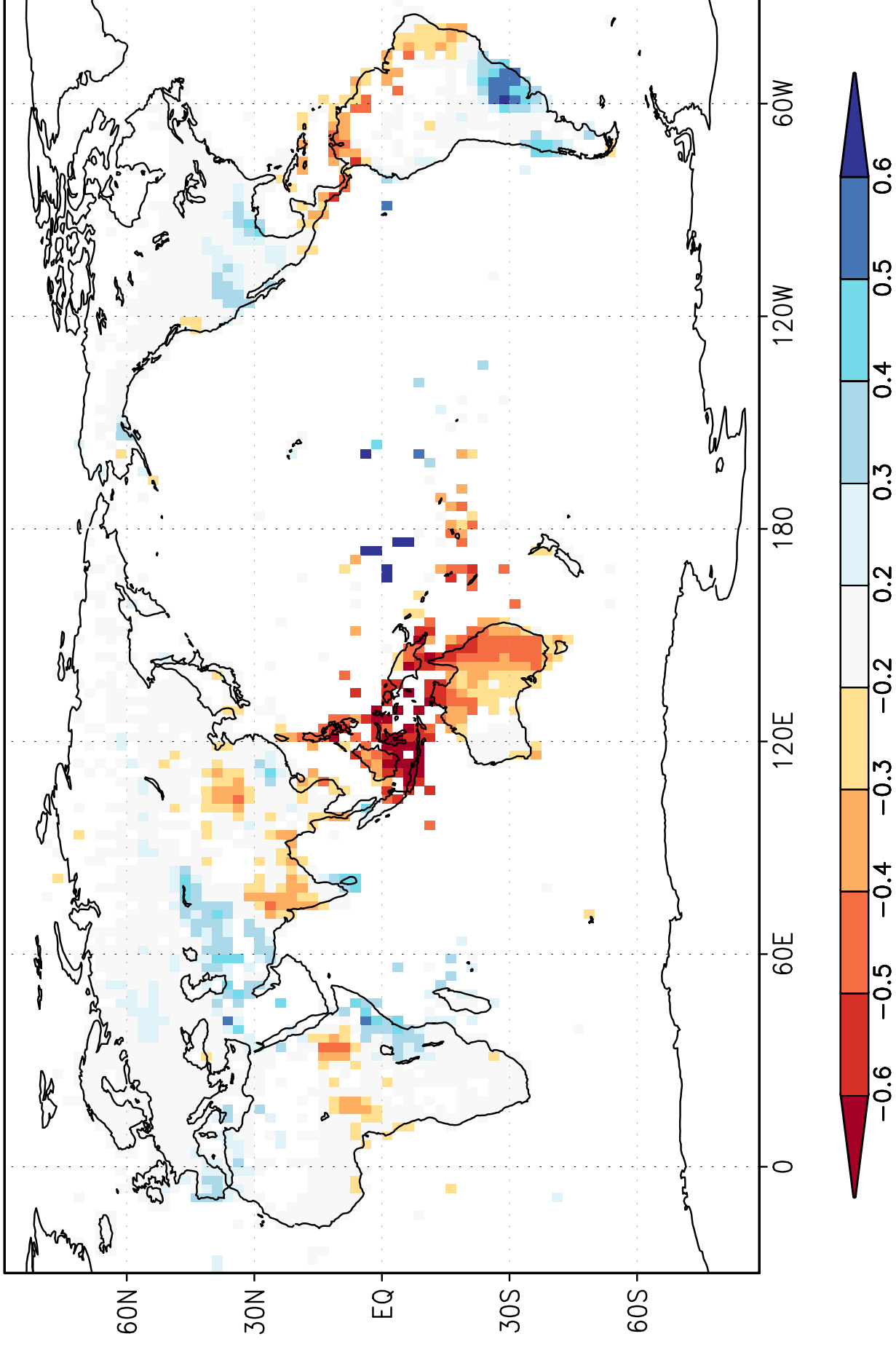
corr Sep–Nov NINO3.4 index with Sep–Nov GPCC V7 2.5 precipitation 1901:2013
